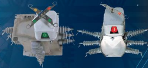
Pole mounted SF6 Load Break Switch (Sectionalizer)
